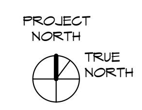
PARTIAL THIRD FLOOR SIGNAGE PLAN - NORTH 1/8" = 1'-0"
